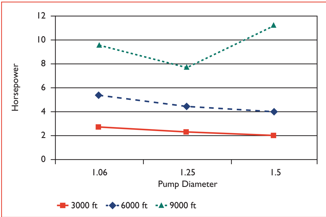
Figure 3. Horsepower Requirement
