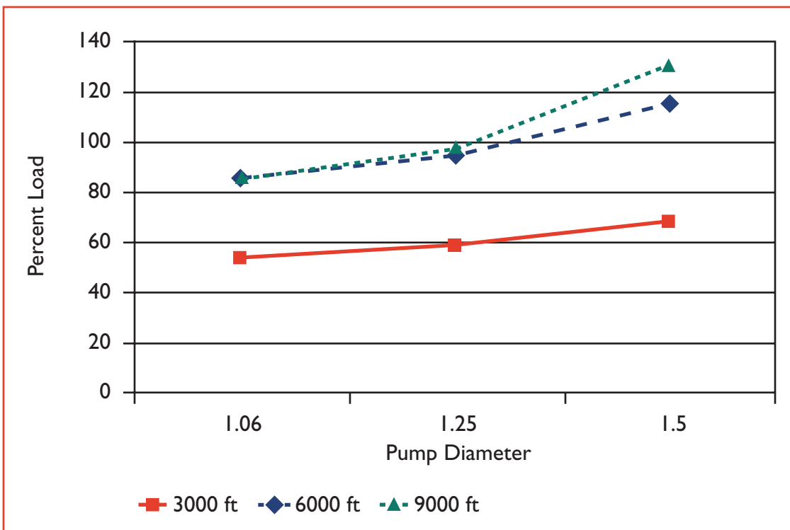
Figure 1. Rod Loading
